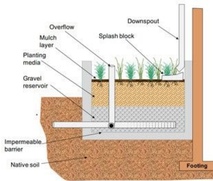
Illustration of a Planter Box
